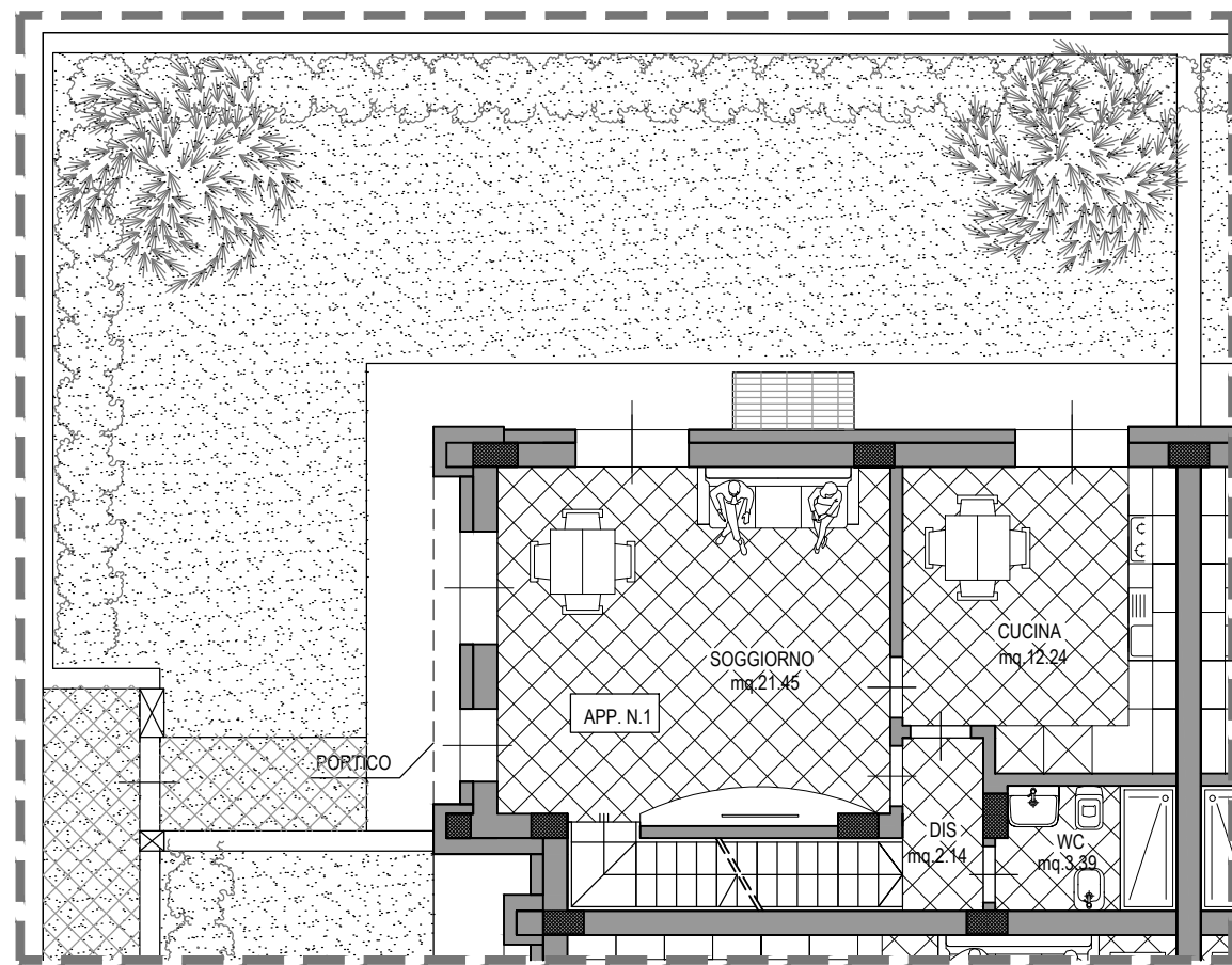
PIANO TERRA
